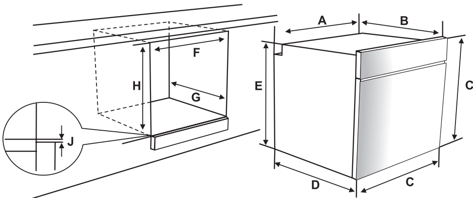
Installation under a worktop
