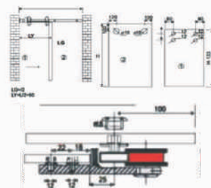
Floor Guide Brass 1 pcs
