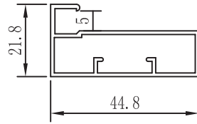
45mm. Aluminum Shutter
