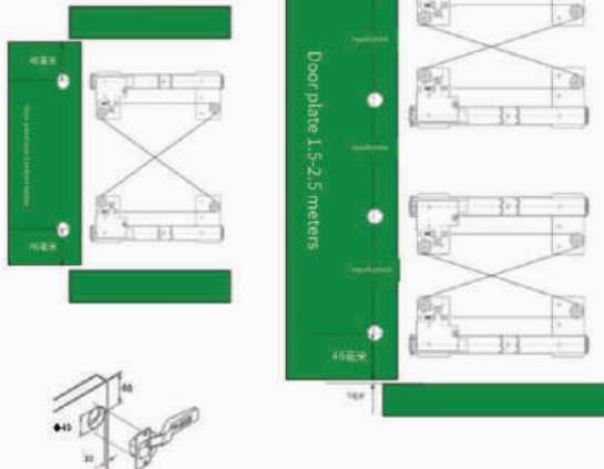
Standard 40mm medium-bend damping hinge (18mm-27mm thickness of door plate)
