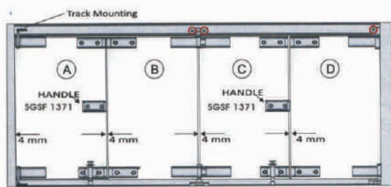
GLASS SLIDING FOLDING SYSTEM SGSF 1361 WITH CENTER OPTIONAL HANDLE
